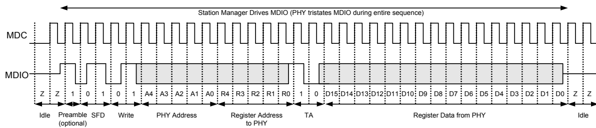
Figure 10. SMI Write Frame
